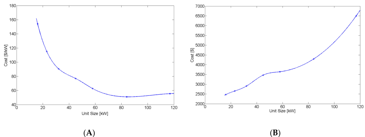
Figure 4. Costs of a gas-fired boiler as a function of its size. (A) cost per kW; (B) cost per unit.
